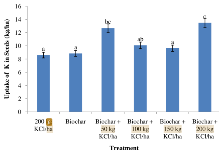
Figure 3. Potassium uptake in the grain of maize at harvest
