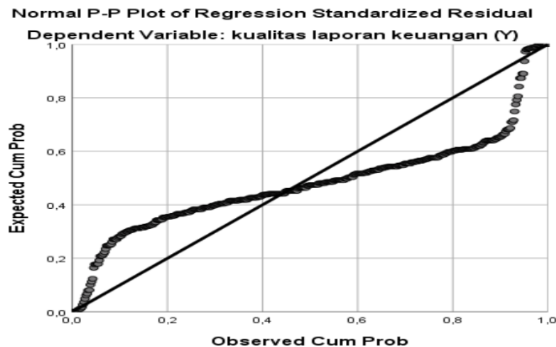
Gambar 1. Hasil Uji Normalitas Probability Plot
