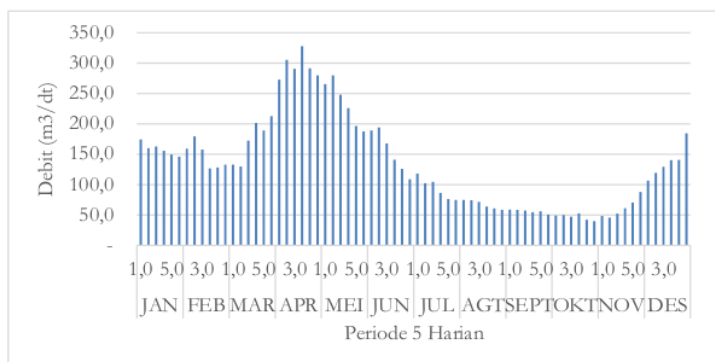
Gambar 2. Debit Andalan (Q80%) Bendung Benteng
