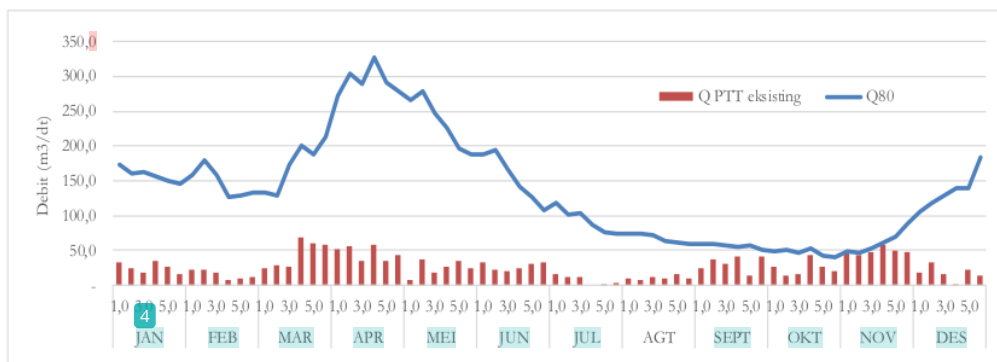
Gambar 6. Neraca Air Optimal PTT Eksisting (Intensitas Tanam 280%)
