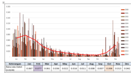
Gambar 6. Debit Bulanan FJ. Mock
