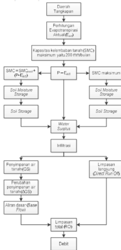
Gambar 2. Diagram Metode FJ. Mock
