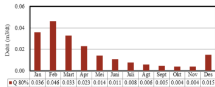
Gambar 7. Debit Andalan Q 80%
